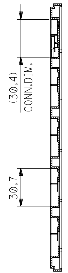
SECT. Y-Y
